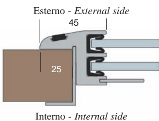
Profilo scorrevole - Sliding profile
