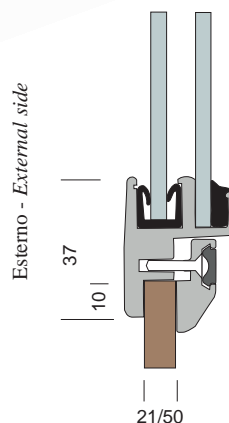
Profilo scorrevole Sliding profile
